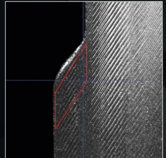
Contour measurement in the flute
