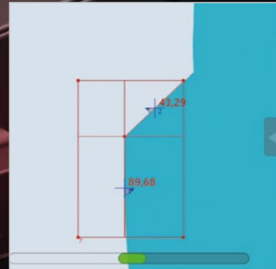
Transmitted light measurement in the profile.
