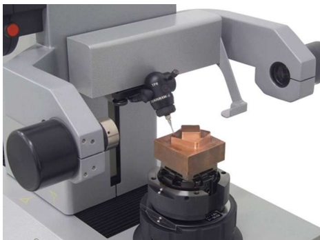
Picture 3: The measuring probe for measuring of the offset in X and Y, the angular offset and the length of electrodes.
